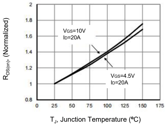
Figure 7. Drain-Source On-Resistance
